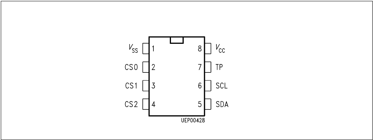
Pin Configuration (top view)
