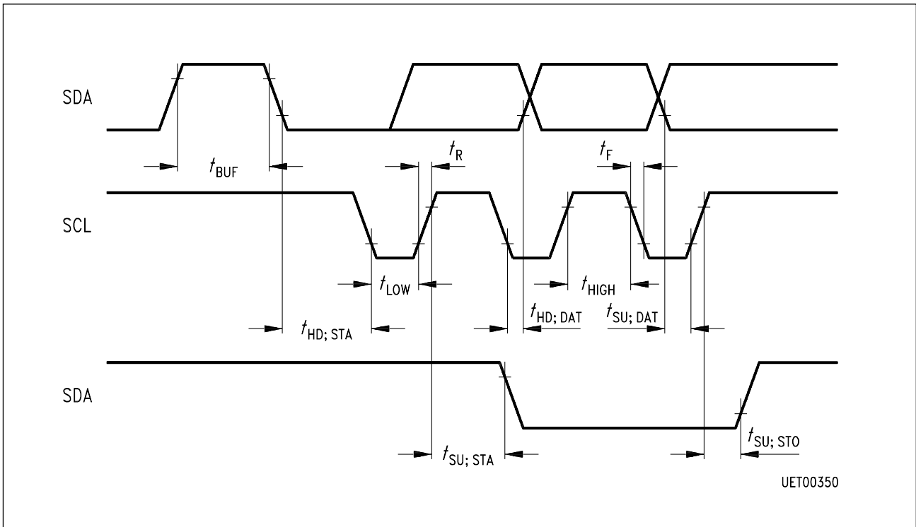
Figure 2 Timing Conditions for the I²C Bus (high-speed mode)
